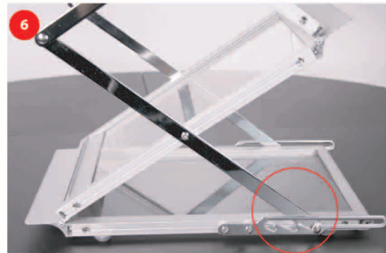
6 POSITION LOCKING PIN AT BOTTOM OF BASE PRIOR TO USING UNIT.
