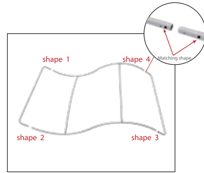
3. Connect corner sections to straight sections with matching shape codes.
